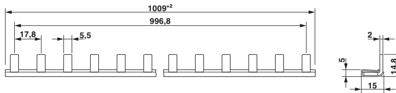
Dimensional drawing
